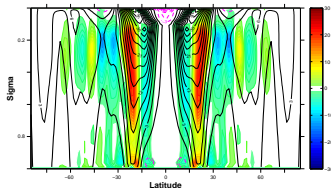
Quasilinear approximation.
